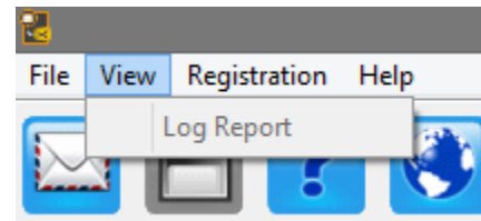
View Menu
