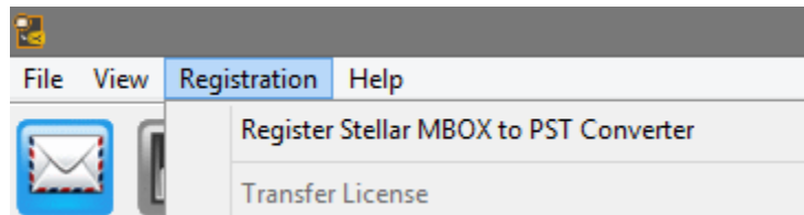
Registration Menu
