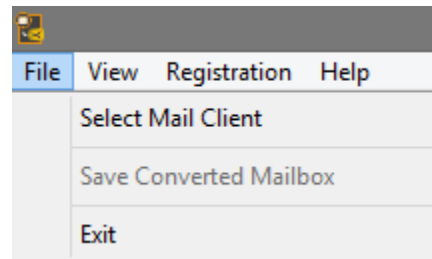
File Menu
